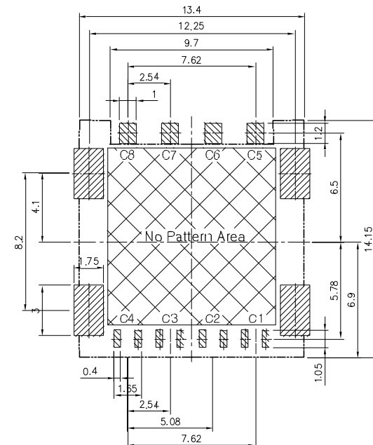
P.C.B LAYOUT (Top View) (General Tolerance +0.05)
