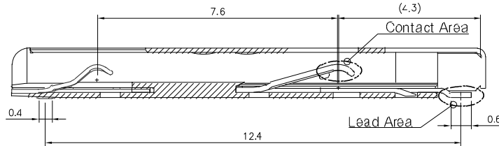
SECT ON A-A' (ZOOM VIEW)
