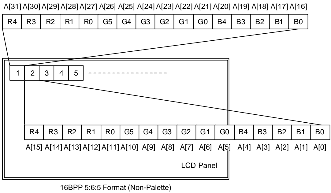
Figure 15-5. 16BPP Display Types (TFT)
