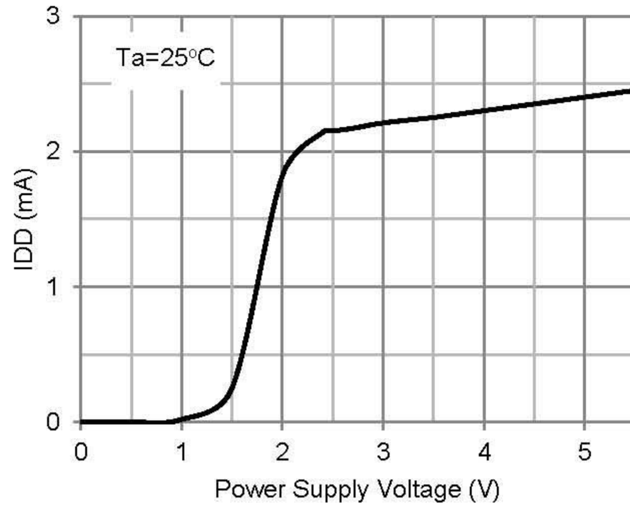
Power Supply Current Consumption
