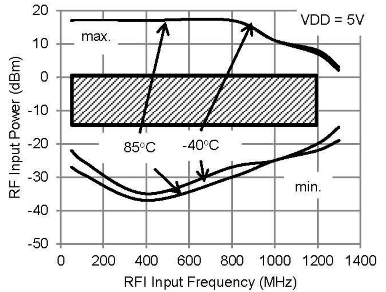
RF Input Sensitivity vs Temperature (64/65 mode)
