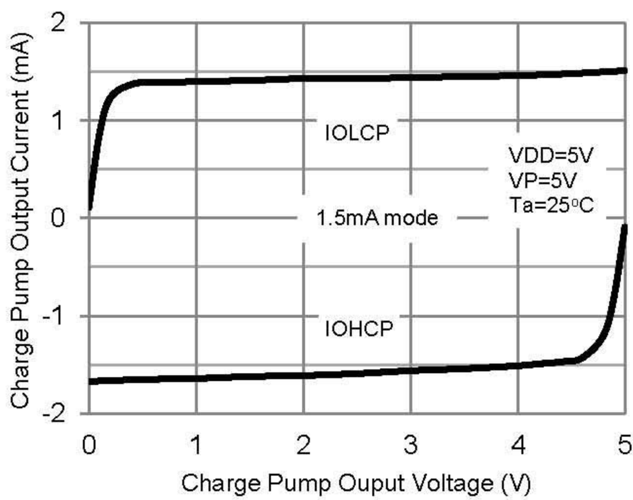
Charge Pump Output Characteristics
