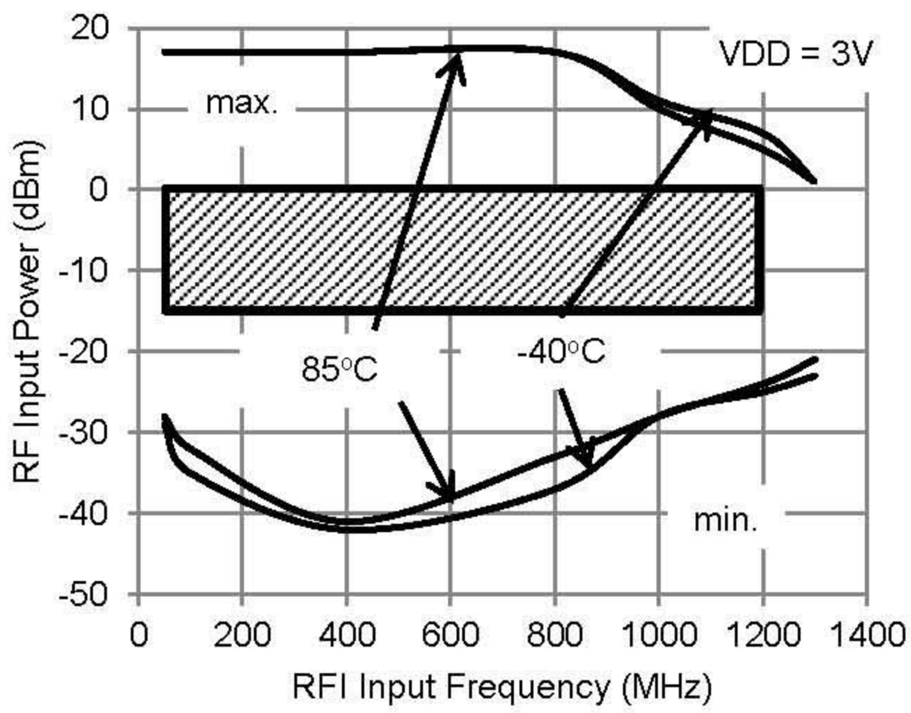
RF Input Sensitivity vs Temperature (64/65 mode)
