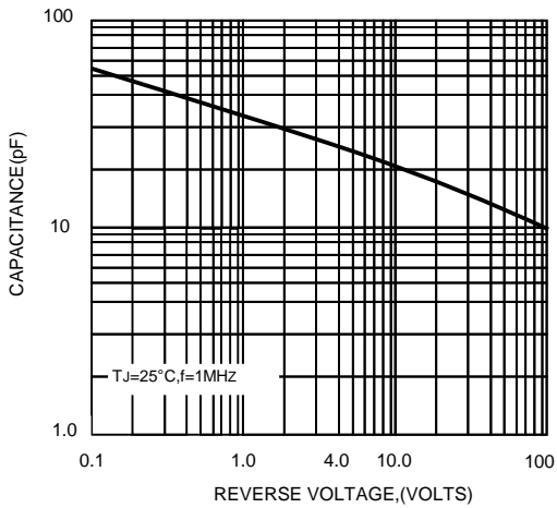
FIG.3-TYPICAL JUNCTION CAPACITANCE
