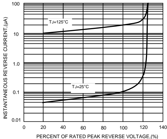
FIG.5-TYPICAL REVERSE CHARACTERISTICS
