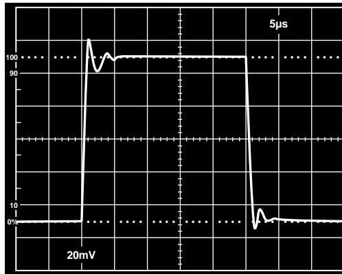
Figure 33. Unity Gain Inverter Small Signal Pulse Response, C_L = 1000 \text{ pF}
