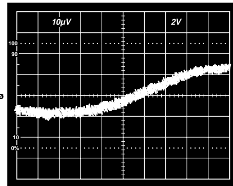
Figure 12. Gain Nonlinearity, G = 1 , R_L = 10\text{ k}\Omega ( 20\ \mu\text{V} = 2\text{ ppm} )
