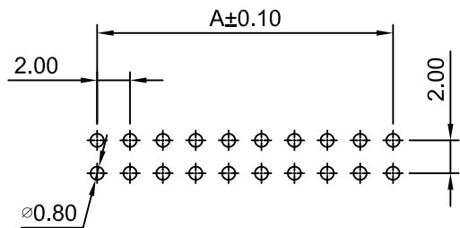
P.C.B LAYOUT TOLERANCE:±0.05
