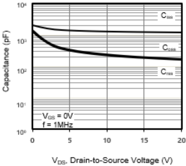
Fig.7 Capacitance
