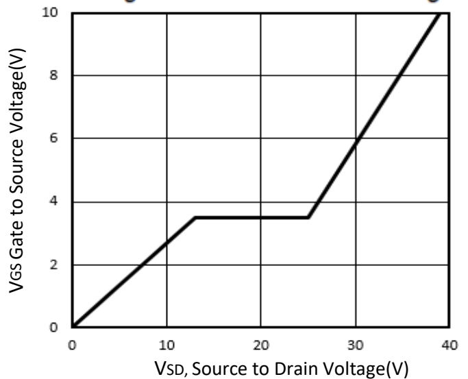
Fig.4 Gate-Charge Characteristics
