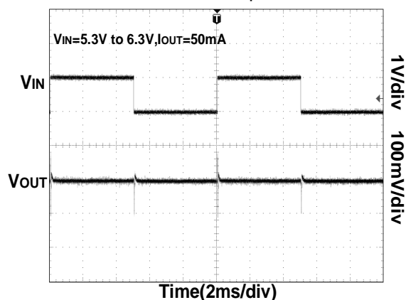
Line-Transient Response
