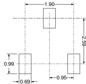
RECOMMENDED LAND PATTERN (Unit: mm)
