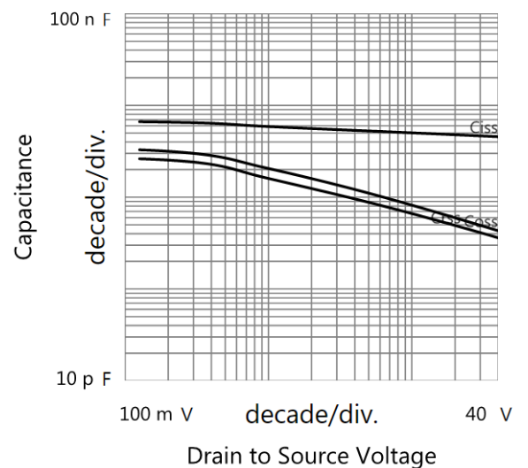
Capacitances
