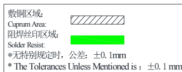
推荐焊盘尺寸 Recommended Soldering Pad
