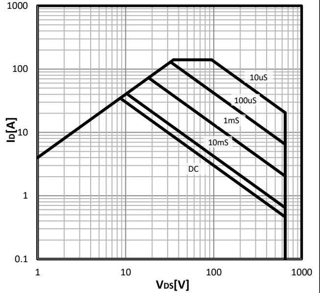
Safe operating area T_C=25\text{ }^\circ\text{C} parameter: tp; TO-247
