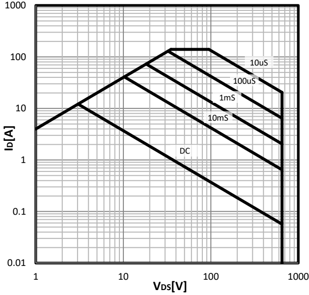
Safe operating area T_C=25\text{ }^\circ\text{C} parameter: tp; TO-220F
