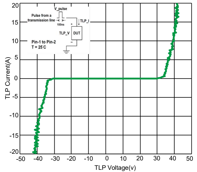
Fig 4. TLP Measurement
