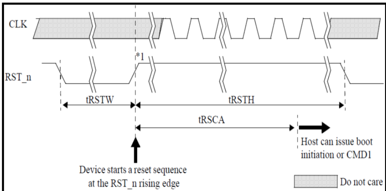
Figure 5-1 H/W Reset Waveform
