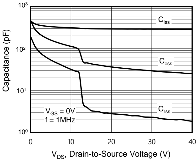
Figure 7. Capacitance
