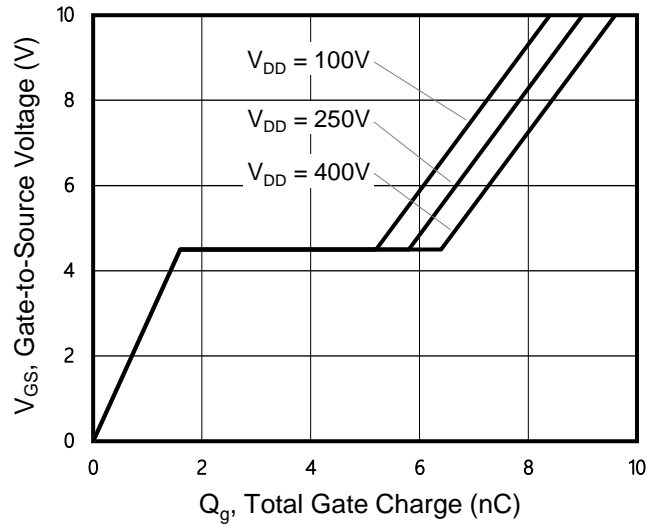
Figure 8. Gate Charge
