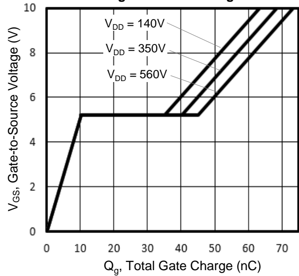
Figure 8. Gate Charge
