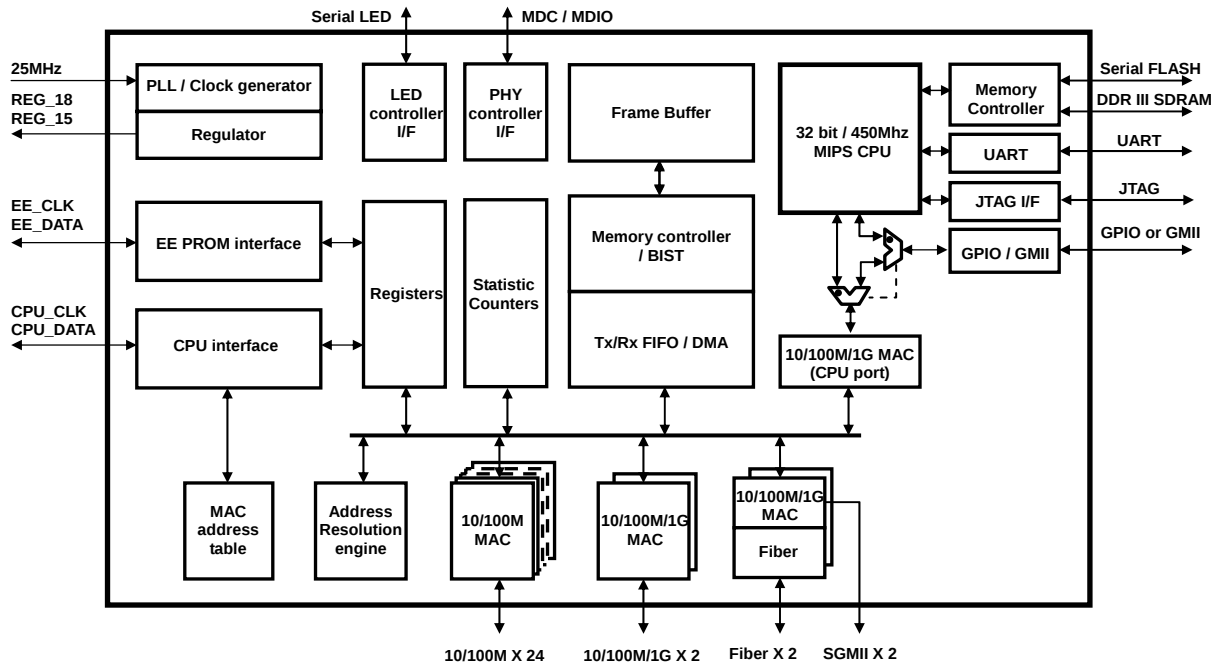
Figure 2 Block Diagram
