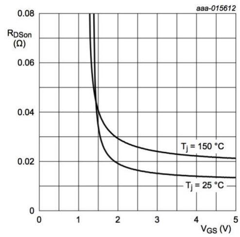
Fig.2 On-Resistance vs. Gate-Source
