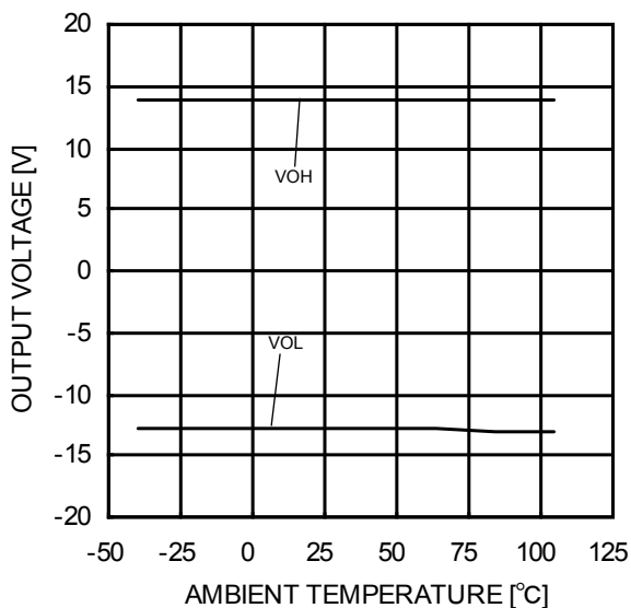
Figure 52. Maximum Output Voltage -Ambient Temperature ( V_{CC}/V_{EE} = +15V/-15V , R_L = 2k\Omega )
