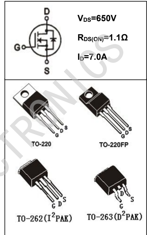
TO-220/220FP/262/263
