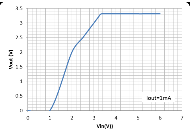
Line Regulation
