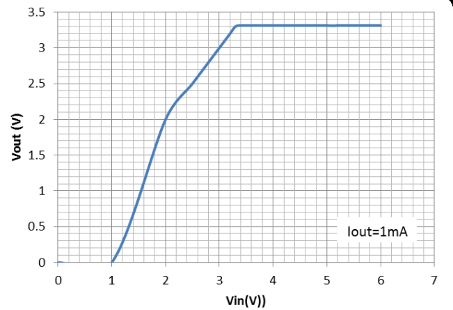
Line Regulation
