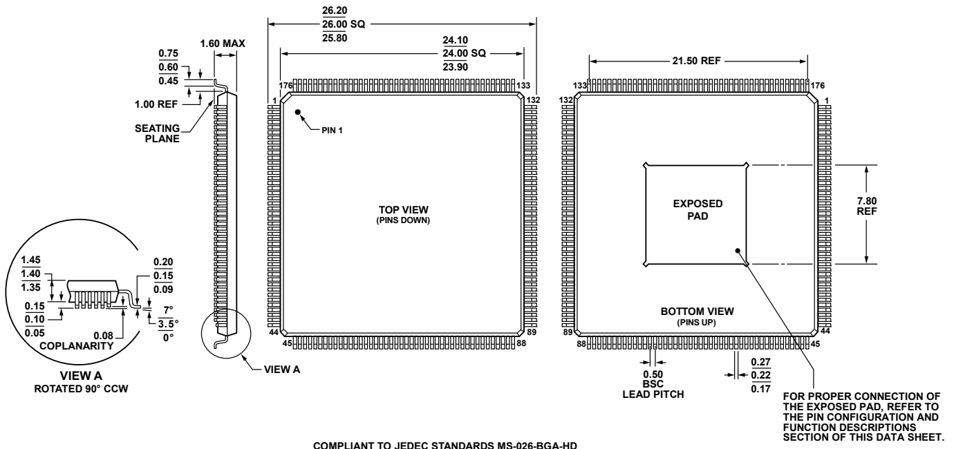
Figure 22. 176-Lead Low Profile Quad Flat Package, Exposed Pad [LQFP_EP] (SW-176-1) Dimensions shown in millimeters
