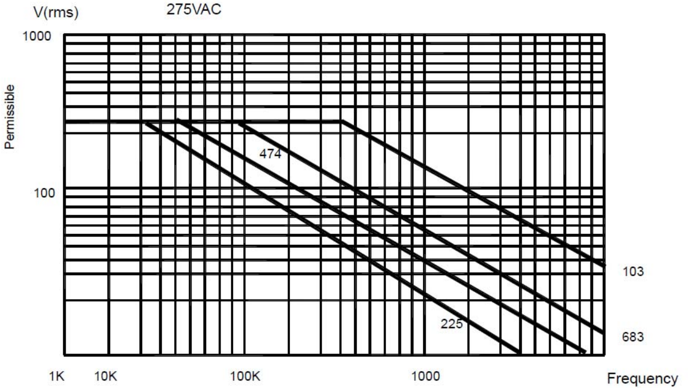
Characteristics of voltage derating to frequency --- MPX
