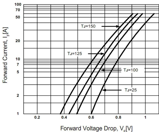
Figure 1. Forward Current Characteristics
