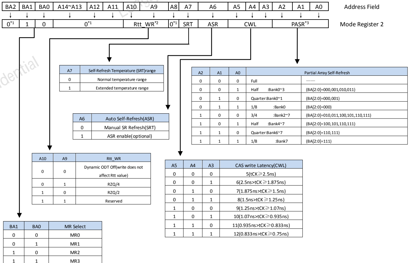
Figure 11 MR2 Programming
