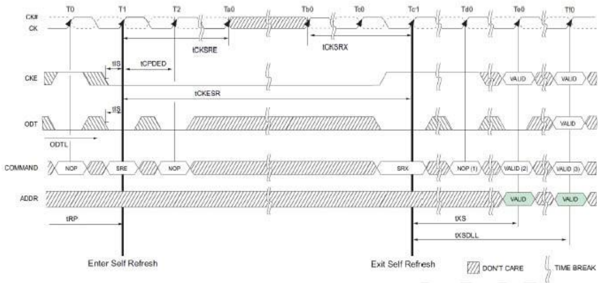
Figure 16 Self-Refresh Entry and Exit Timing
