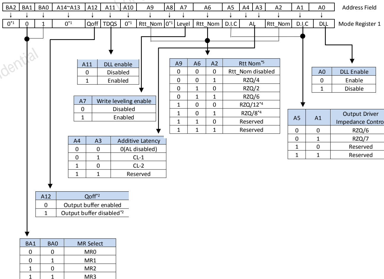
Figure 10 MR1 Programming
