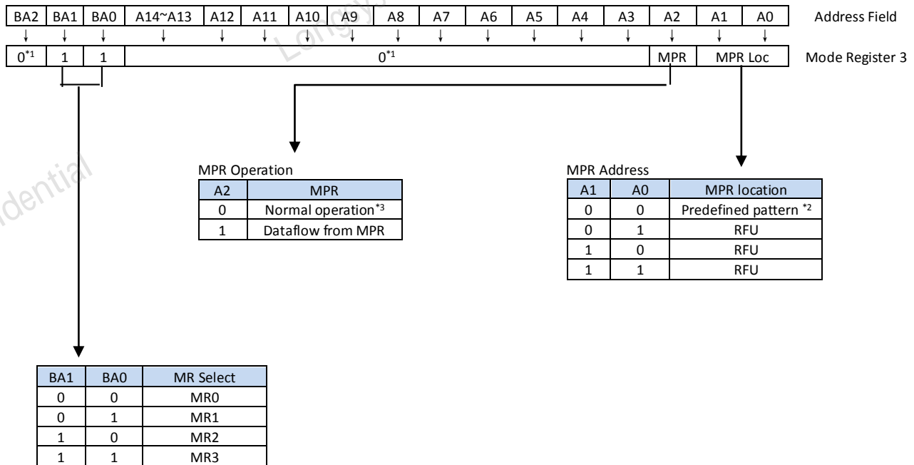
Figure 12 MR3 Programming
