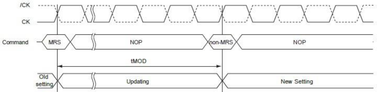
Figure 8 t_{MOD} Timing
