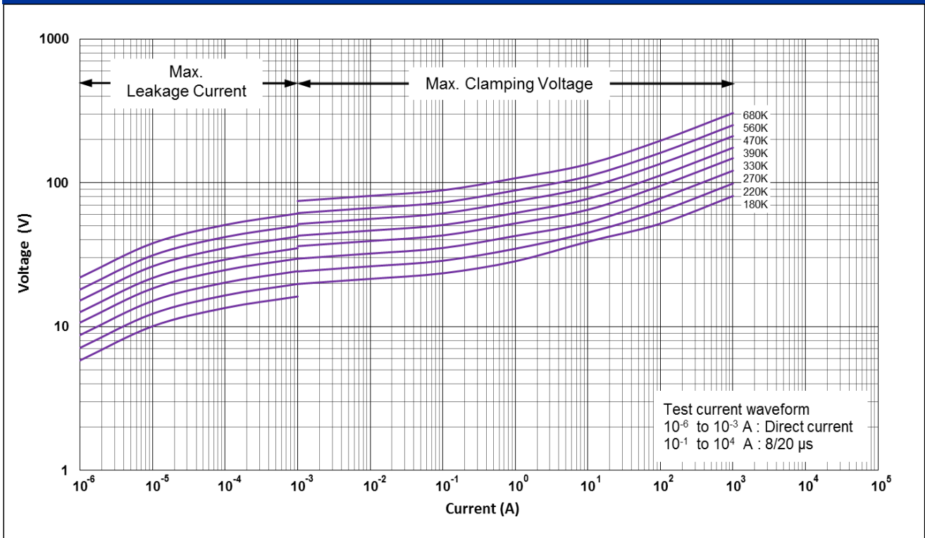
CNR-14D180K to CNR-14D680K V-I Curves
