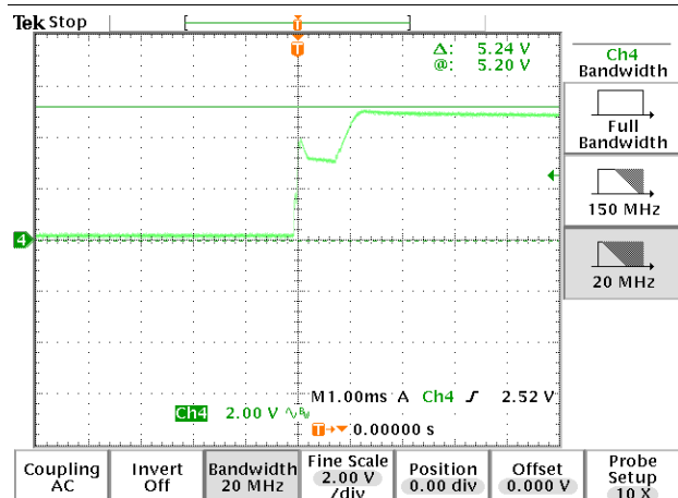
STARTUP (3.3V IN 5V 500MA OUT)
