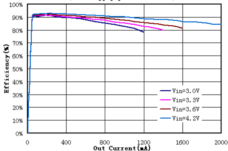
Efficiency vs. Out Current (Vout=5.0V) (Vout supply power to DC-DC)
