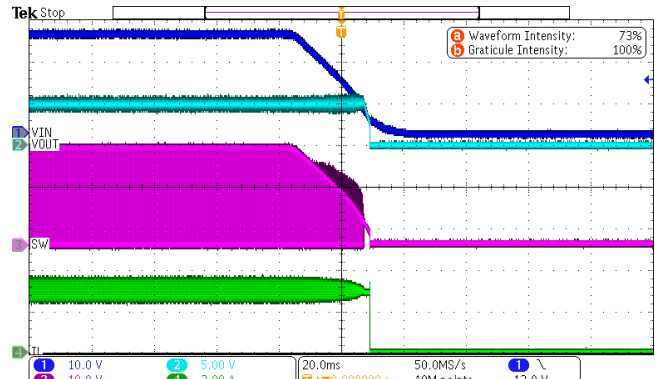
Figure 15. Power Down VIN=24V, VOUT=5V, IOUT=3A
