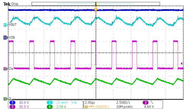
Figure 13. SW node waveform and Output Ripple VIN=24V, IOUT=3A
