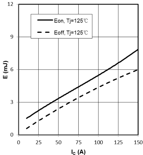
Fig 4. switching losses IGBT, E_{on}=f(I_c), E_{off}=f(I_c) , V_{GE}=\pm 15V, R_{Gon}=7.5\Omega, R_{Goff}=7.5\Omega, V_{CE}=600V
