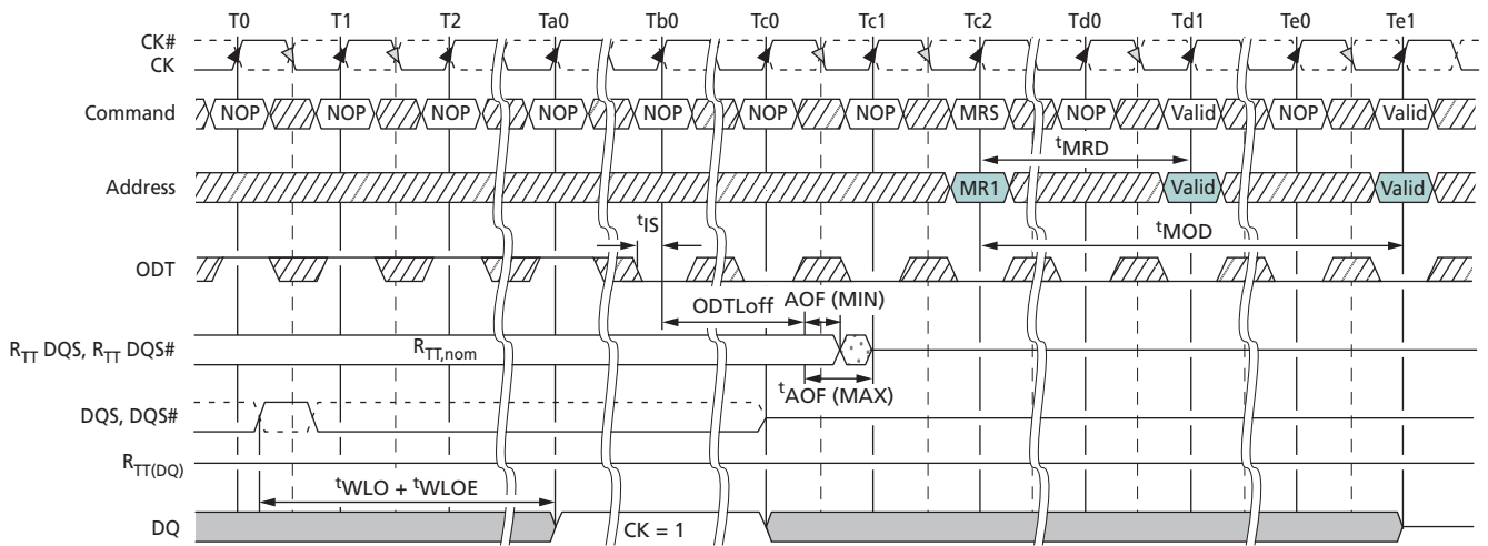
Figure 49: Write Leveling Exit Procedure
