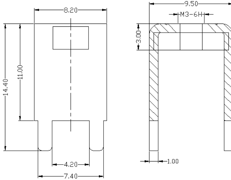
外形尺寸 (Shape Dimension)
