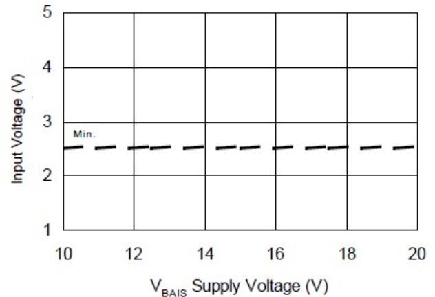
Figure 9B. Logic "1" Input Voltage vs. Supply Voltage
