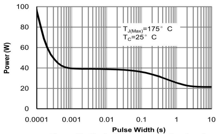
Figure 10: Single Pulse Power Rating Junction-Case (Note F)
