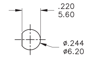
PANEL MOUNTING
