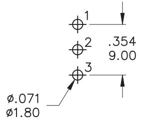
P.C. MOUNTING
