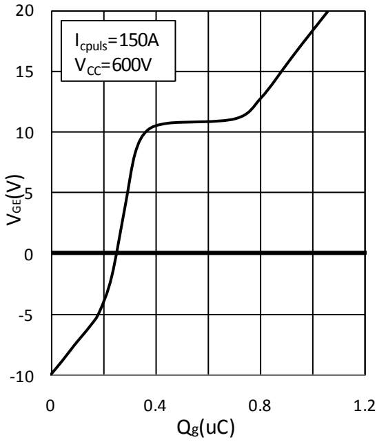
Fig.13 Typ. Gate Charge Characteristics
