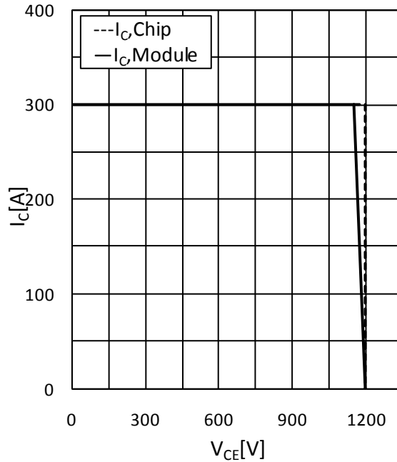
Fig.16 Reverse Bias Safe Operating Area (RBSOA)
