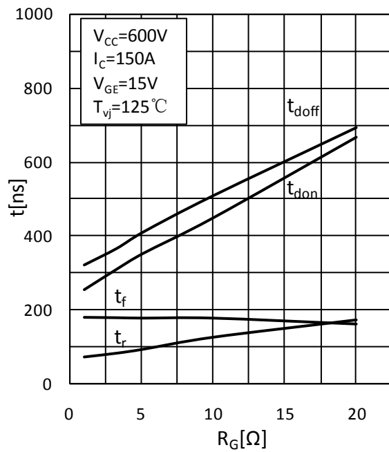
Fig.8 Typ. Switching Times vs. Gate Resistor
