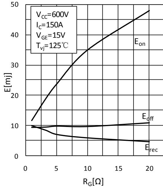
Fig.6 Switching Loss vs. Gate Resistor
