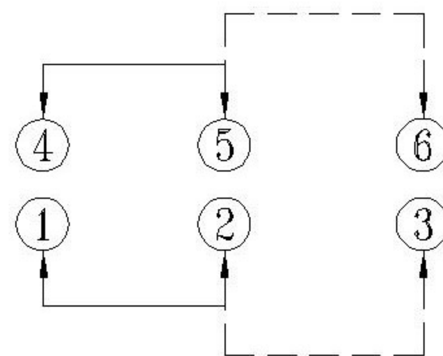
SCHEMATIC (NON-SHORTING)
