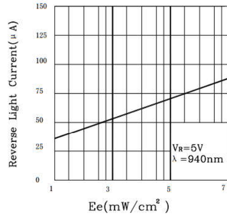
Fig. 4 Reverse Light Current vs. Ee
