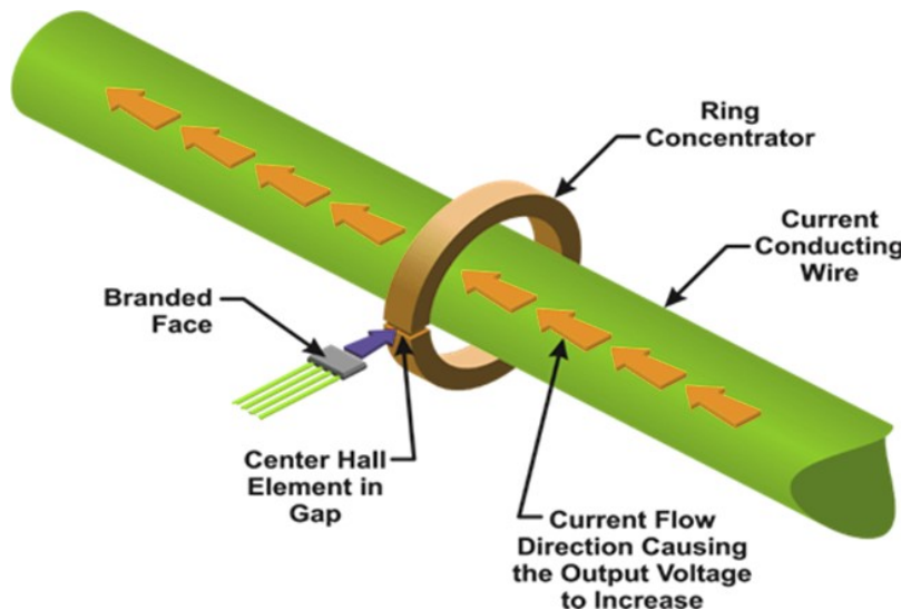
Figure 7: Sensor in Ring Concentrator
