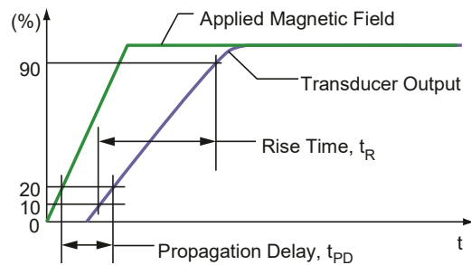
Figure 2: Propagation Delay and Rise Time Definitions
