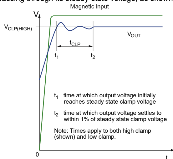
Figure 4: Delay to Clamp Definition
