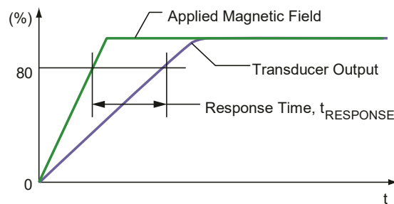
Figure 3: Response Time Definition
