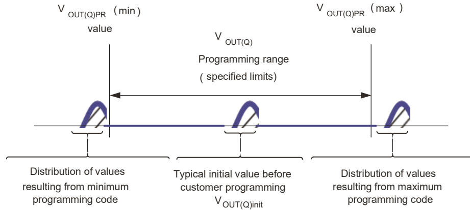
Figure 5: Quiescent Voltage Output Range Definition
