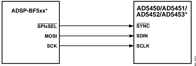
Figure 58. ADSP-BF5xx-to-AD5450/AD5451/AD5452/AD5453 Interface
