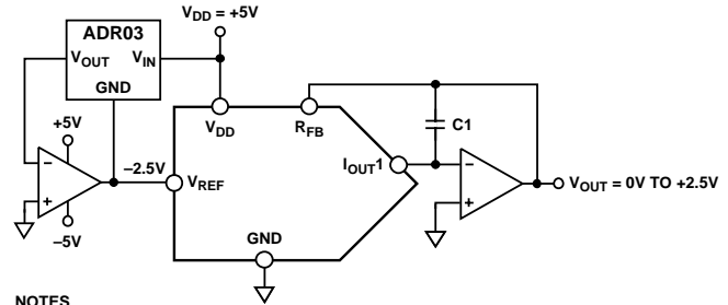
Figure 47. Positive Output Voltage with Minimum Components
