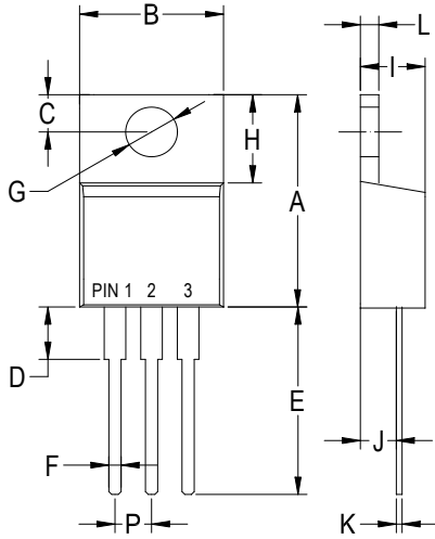
TO-220AB
