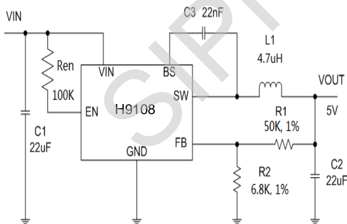
Figure 1. Basic Application Circuit For VOUT=5V
