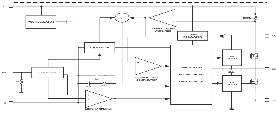
Figure 2. H9108 Block Diagram
