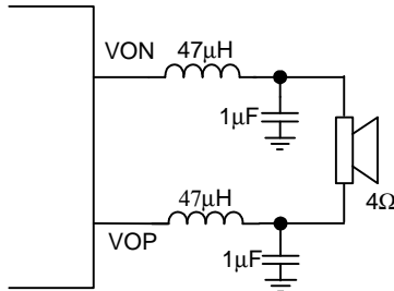
Figure 3. LC output filter
