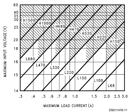
FIGURE 5. LM2576(HV)-12
