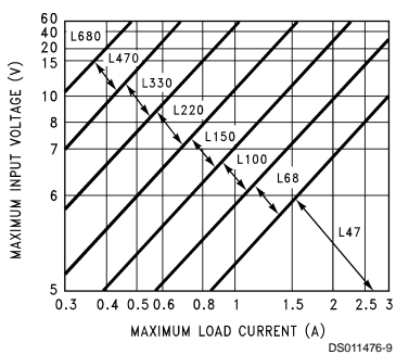
FIGURE 3. LM2576(HV)-3.3
