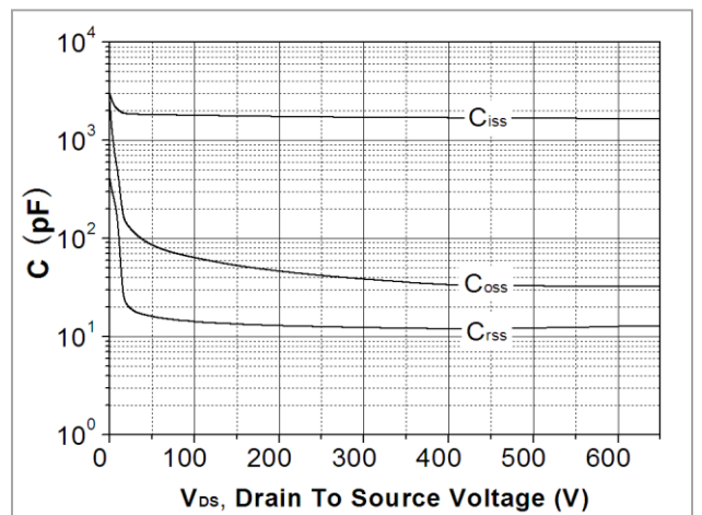
Fig.12. Capacitance Characteristics
